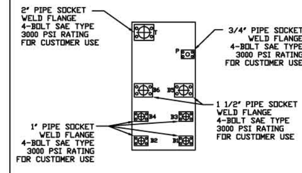
HEADER - FLANGES SPECIFICATION
