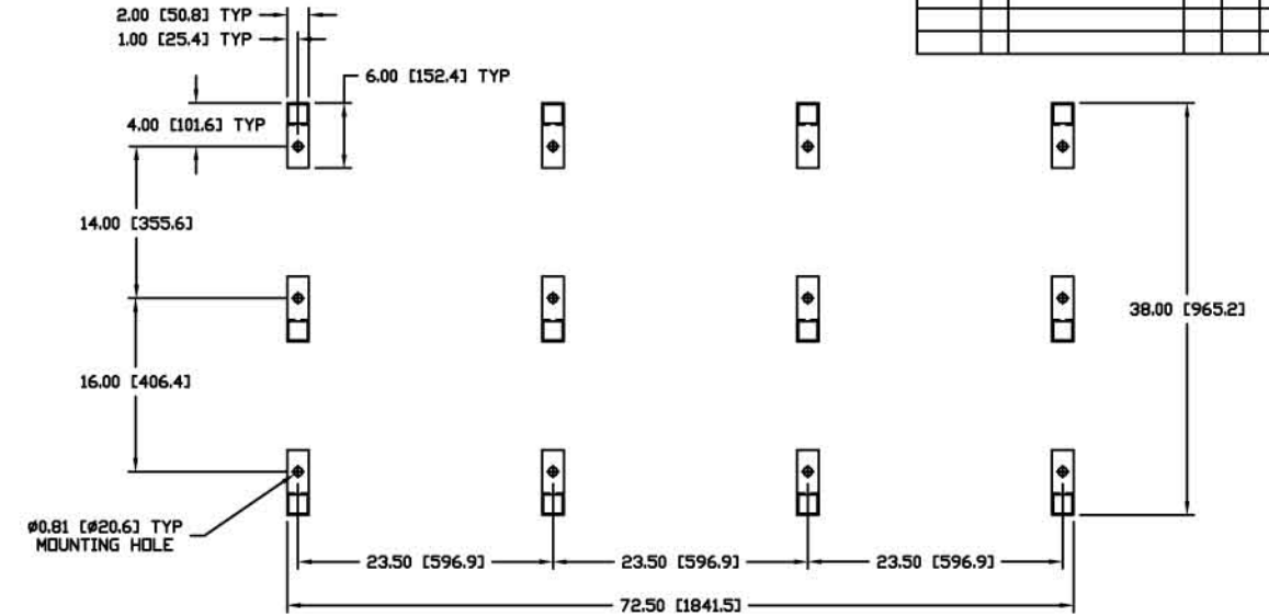
VIEW "A" MOUNTING LEGS
